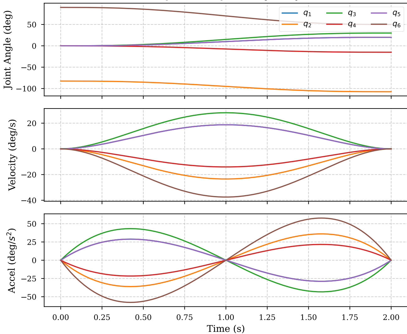
Minimum-Jerk Multi-Joint Trajectory Profile
